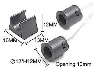
Sensor Head
